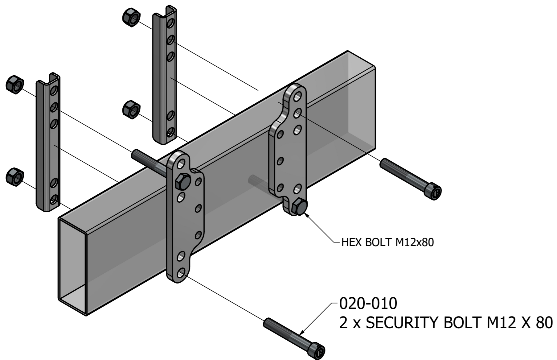
MOUNTING SYSTEM
